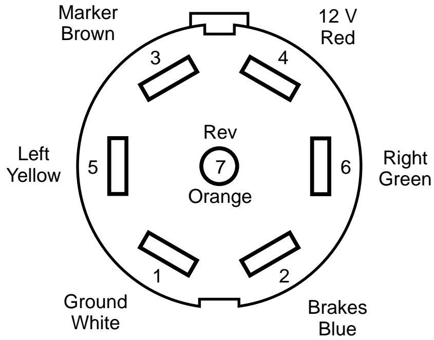
Front of Vehicle Socket / Back of Trailer Plug
