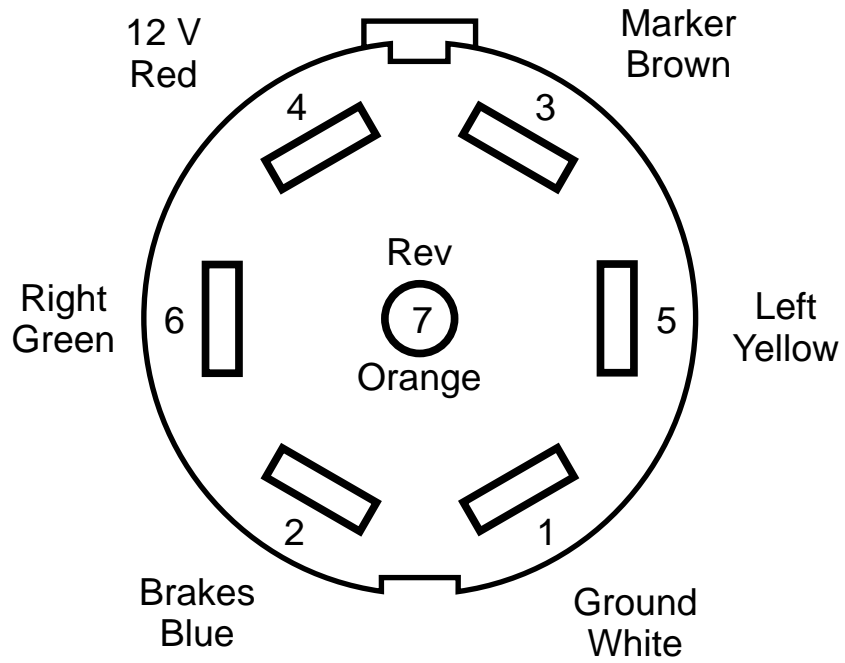
Front of Trailer Plug / Back of Vehicle Socket
